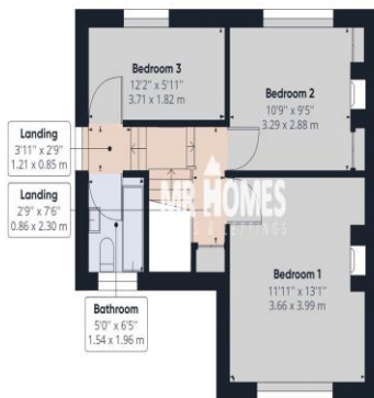
Floor 1
